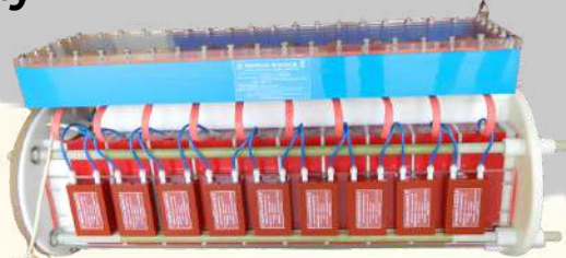
Marx Generator Z/28/19
